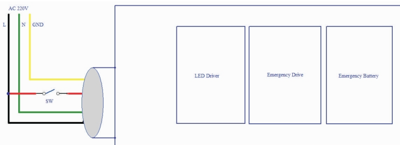
LED emergency lights external wiring diagram
